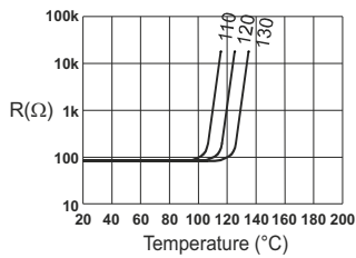
Typical resistance of PTC vs * temperature characteristics graph
