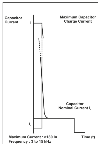
Capacitor inrush current chart
