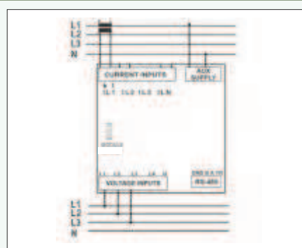
MPR-4 Series (3 Phase connection in balanced network)
