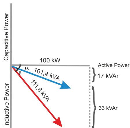
Reactive Power
