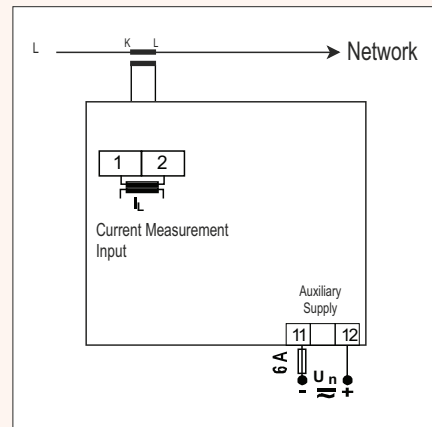
EPM-14 PR19 (96x96)
