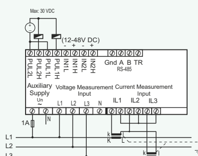
EPR-04S (3 Phase without Neutral with Aron)
