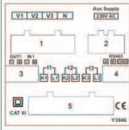
MPR-3 Series (3 Phase connection in balanced networks)
