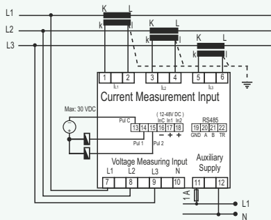
EPR-04S (3 Phase without Neutral)
