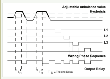
Function Diagram
