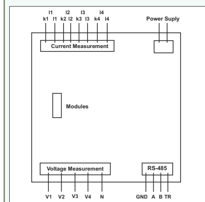
MPR-4 Series (3 Phase connection in balanced network)
