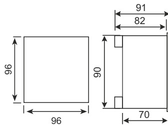
TYPE PR 19 (96x96)
