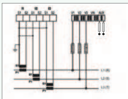
MPR-3 Series (3 Phase connection in balanced networks)
