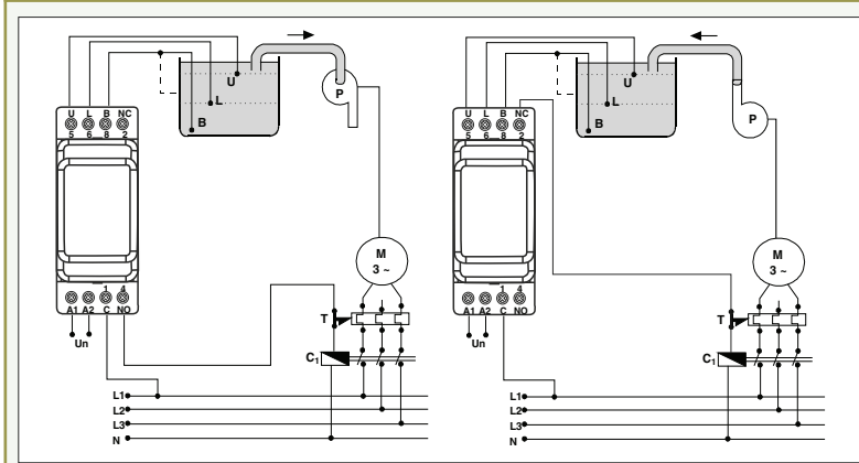
Connection Diagram
