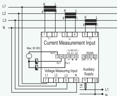
EPR-04S (3 Phase Neutral)
