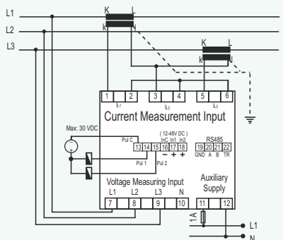
EPR-04S (3 Phase without Neutral with Aron)
