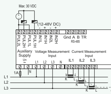
EPR-04S (3 Phase without Neutral)
