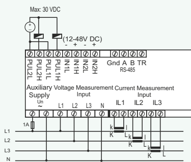
EPR-04S (3 Phase Neutral)
