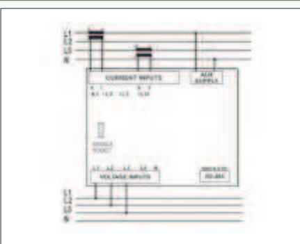
MPR-4 Series (3 Phase, Aron connection)
