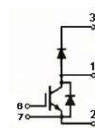
Circuit 2(Boost Chopper)
