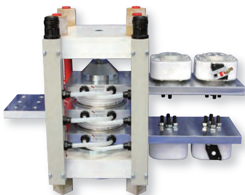
E Water cooled power assembly for high power supplies
