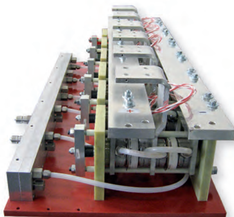
H Controlled three phase bridge cooled by Deionized Water
